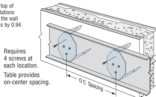
Typical Steel Ledger Installation with ICFVL (Minimum 16 gauge, 54 mil steel ledger)
