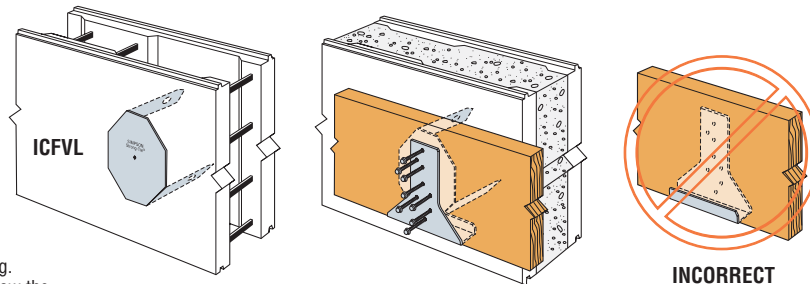
Typical Wood Ledger Installation with ICFVL and ICFVL-W (ICFVL-CW for LVL ledger similar)
