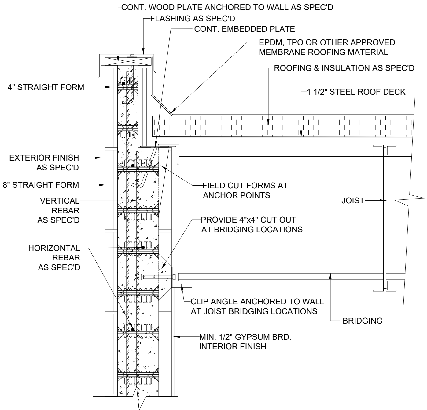
1 STEEL JOIST ROOF DETAIL SIDE WALL PARAPET 8 INCH TO 4 INCH
