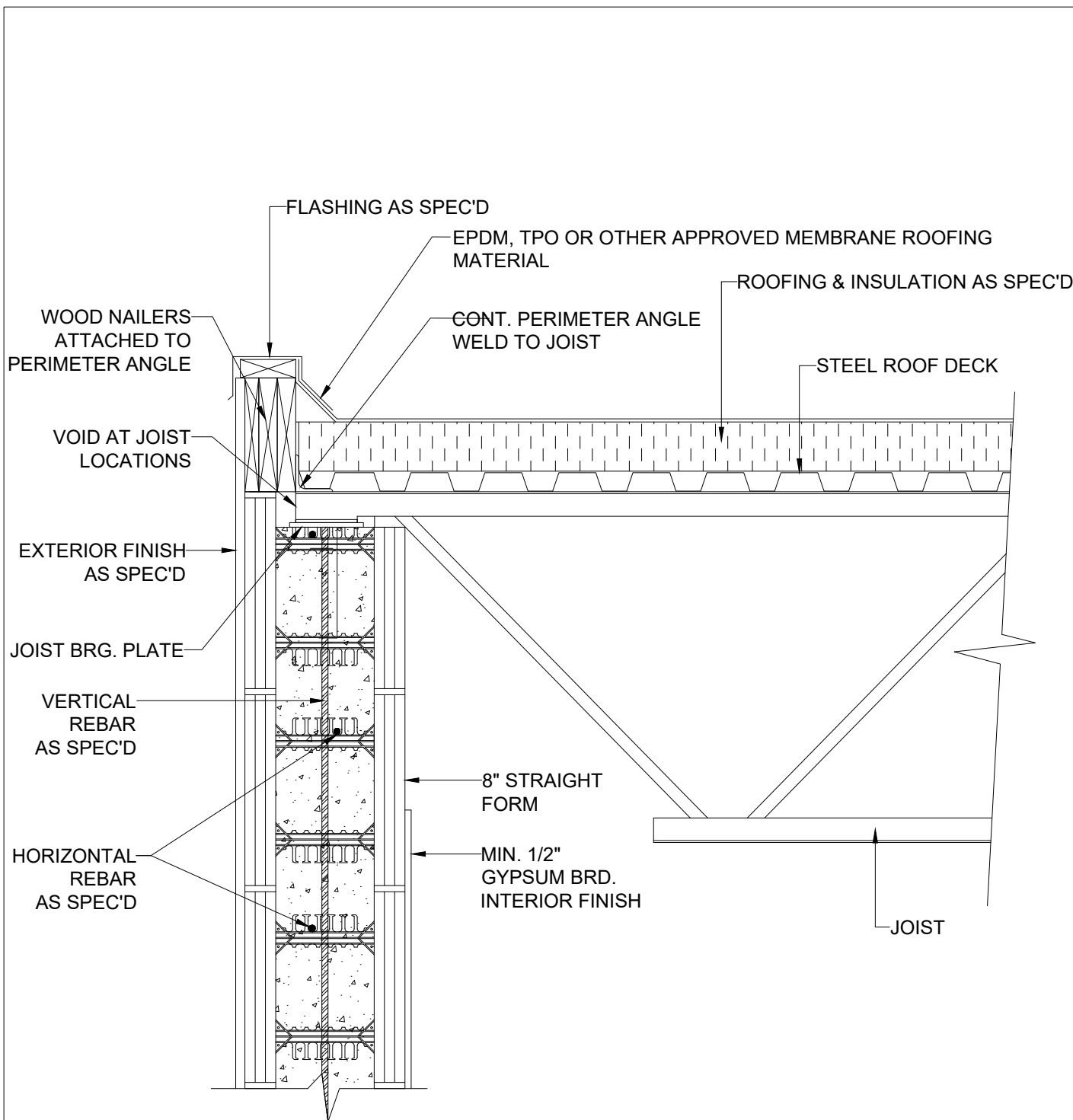
1 STEEL JOIST ROOF DETAIL BEARING WALL, NO PARAPET 8 INCH
