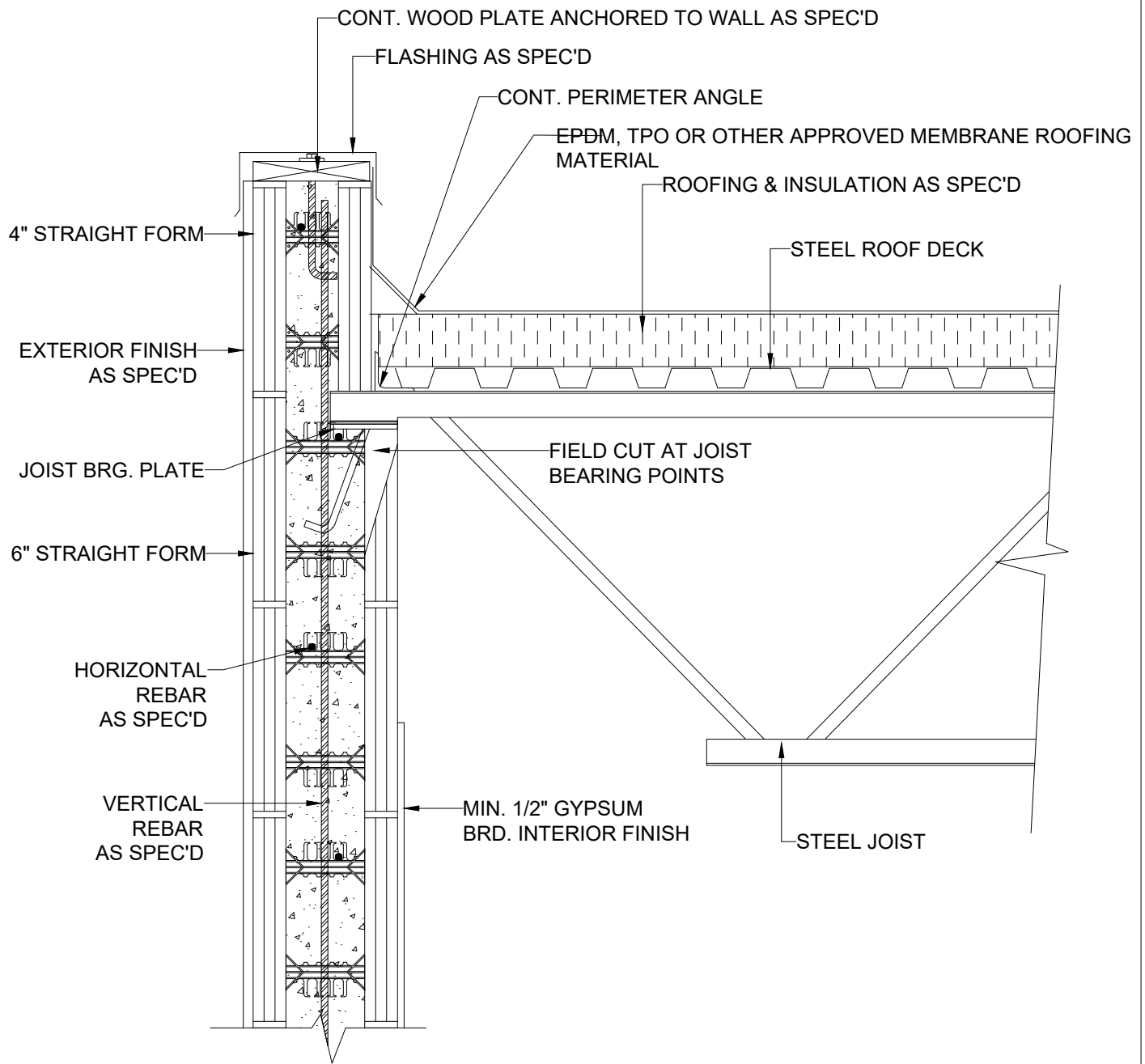
1 STEEL JOIST ROOF DETAIL BEARING WALL WITH PARAPET 6 INCH TO 4 INCH
