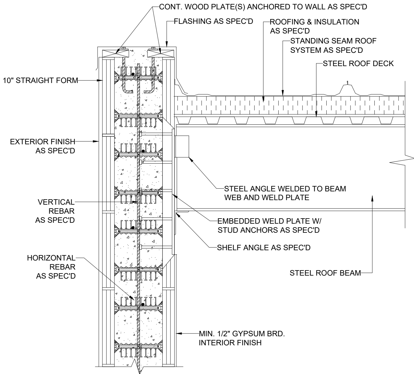
1 STEEL JOIST ROOF DETAIL BEARING WALL BEAM FACE MOUNTED 10 INCH
