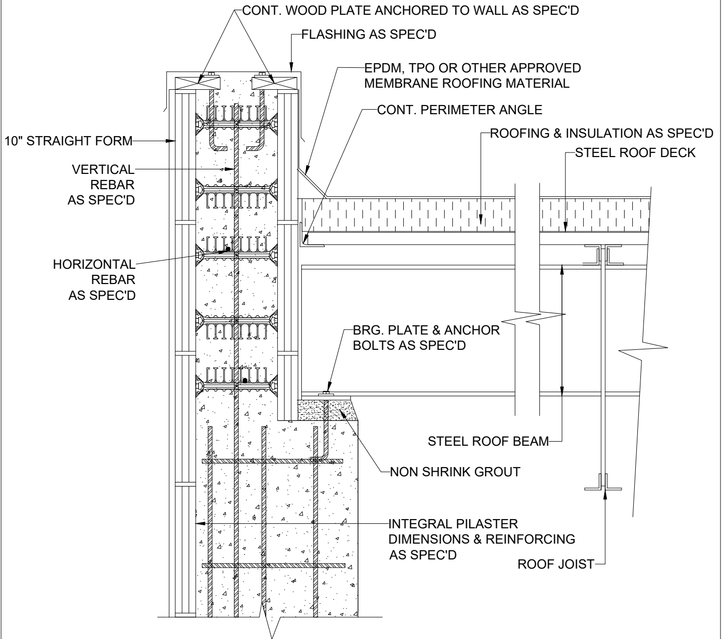
1 ROOM BEAM BEARING ON INTEGRAL PILASTER 10 INCH
