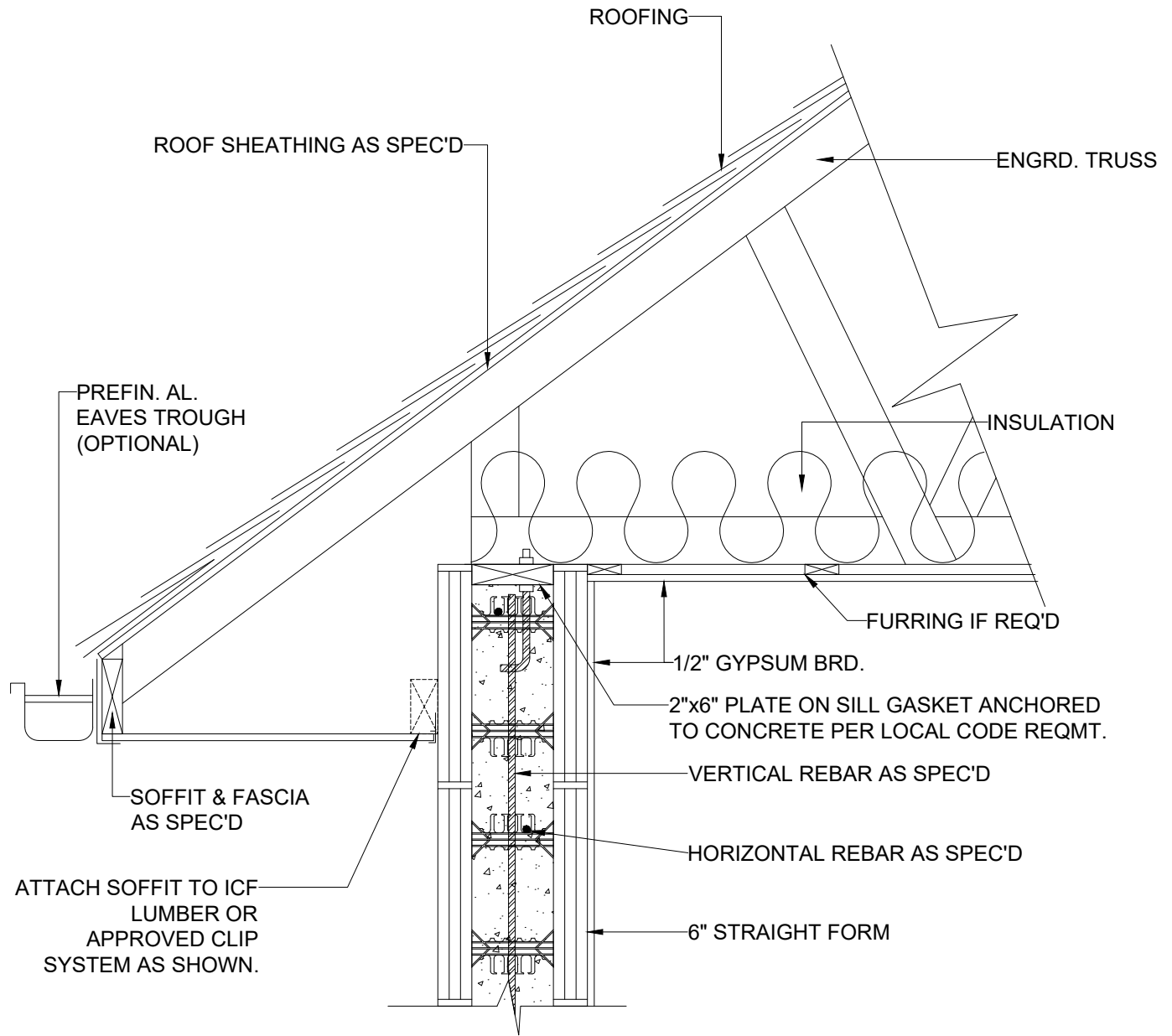
1 EAVE ROOF TRUSS, LOW UPLIFT CONNECTION 6 INCH
