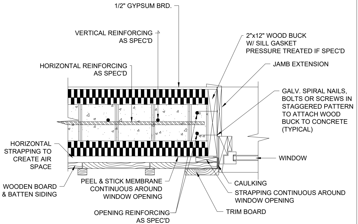
○ WINDOW JAMB DETAIL, WOOD BUCK, BOARD & BATTEN EXTERIOR 6 INCH
