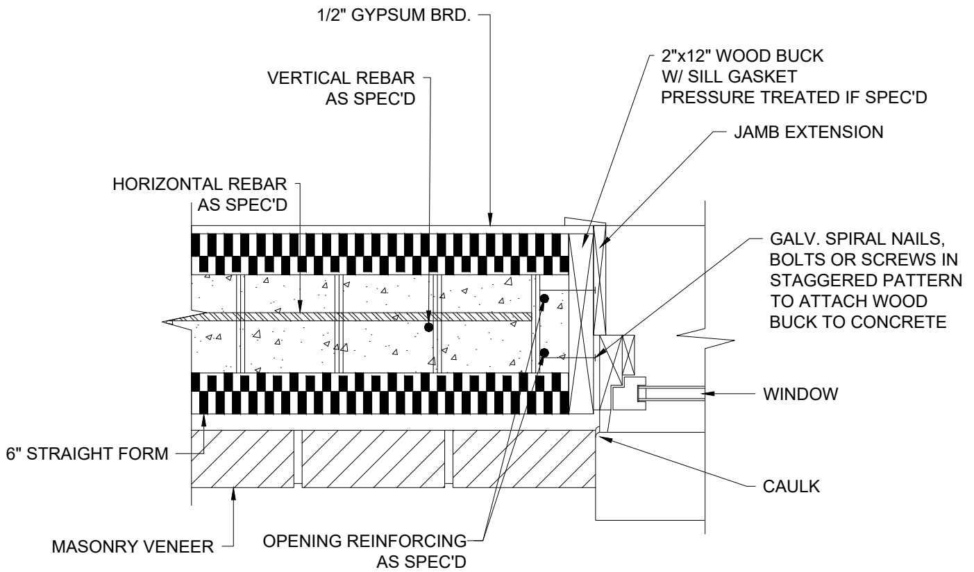
1 WINDOW JAMB DETAIL 6 INCH
