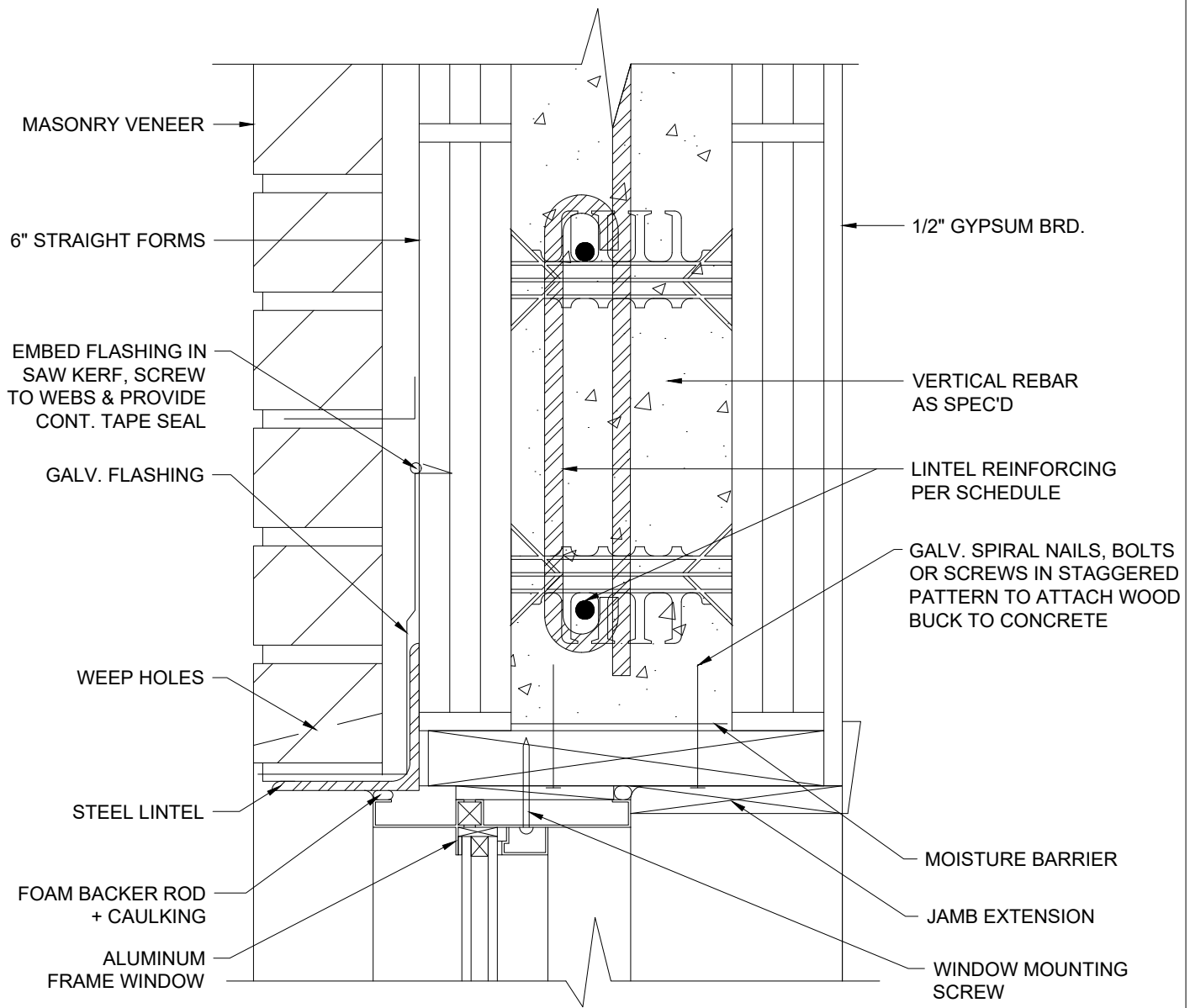
1 WINDOW HEAD DETAIL 6 INCH
