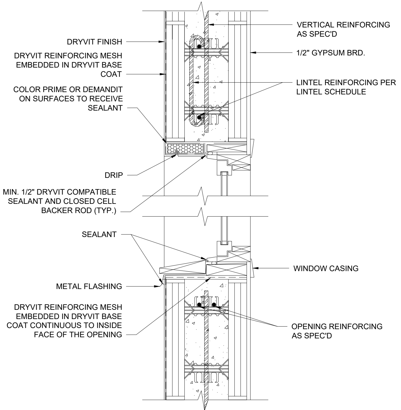
1 DRYVIT WINDOW HEAD/SILL DETAIL 6 INCH
