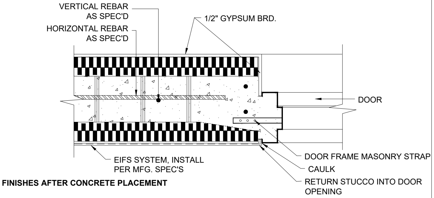
1 STEEL FRAME DOOR JAMB DETAIL 6 INCH
