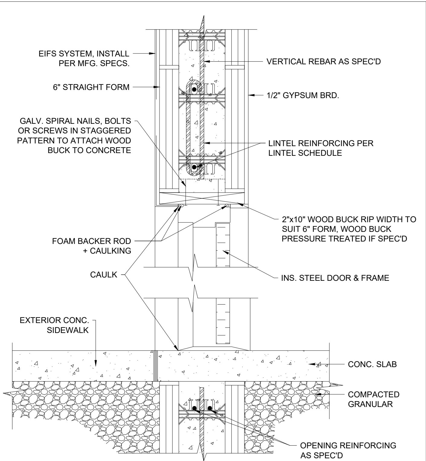
1 DOOR HEAD SILL DETAIL 6 INCH
