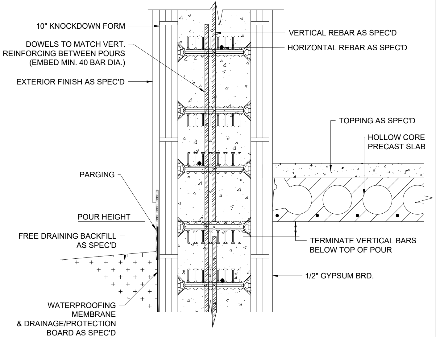
1 HOLLOW CORE PRECAST FLOOR SLAB 10 INCH
