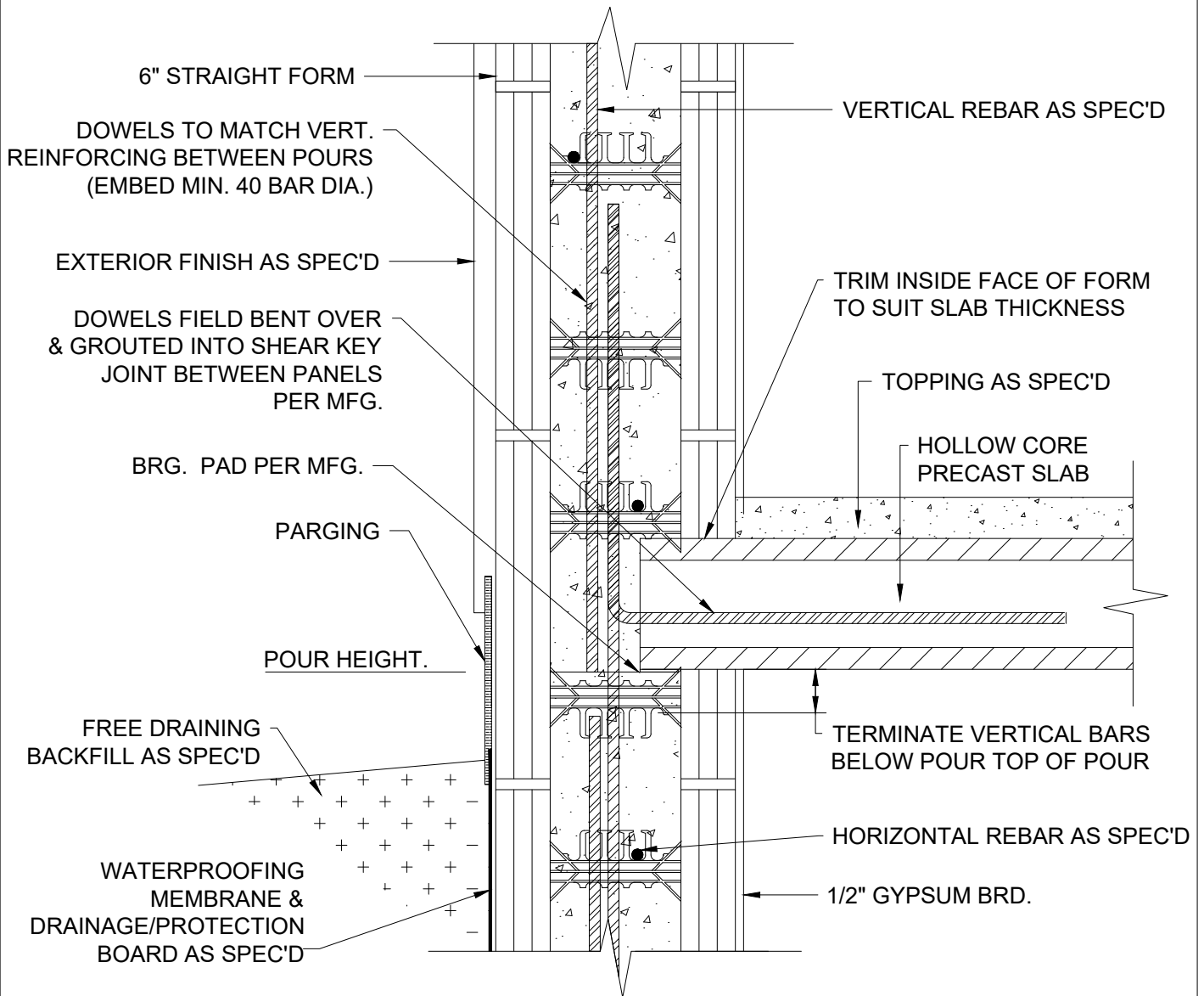
1 HOLLOW CORE PRECAST FLOOR SLAB 6 INCH
