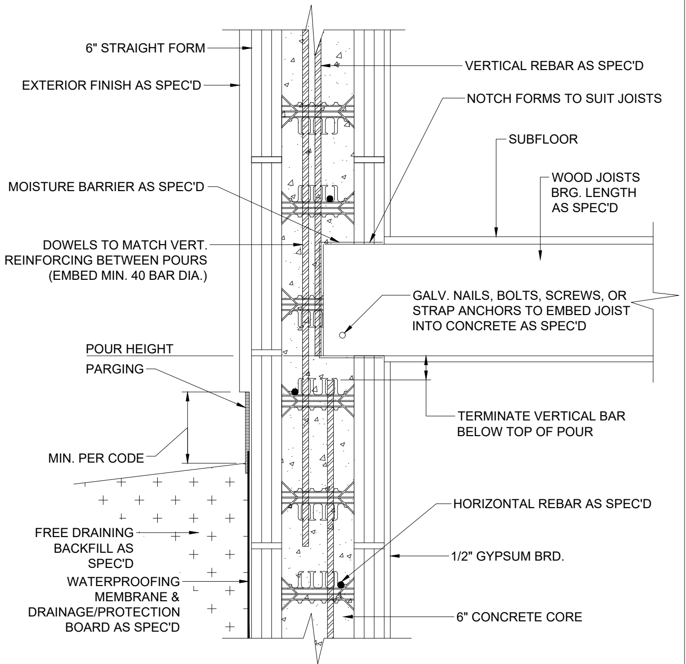
1 EMBEDDED JOIST CONNECTION 6 INCH
