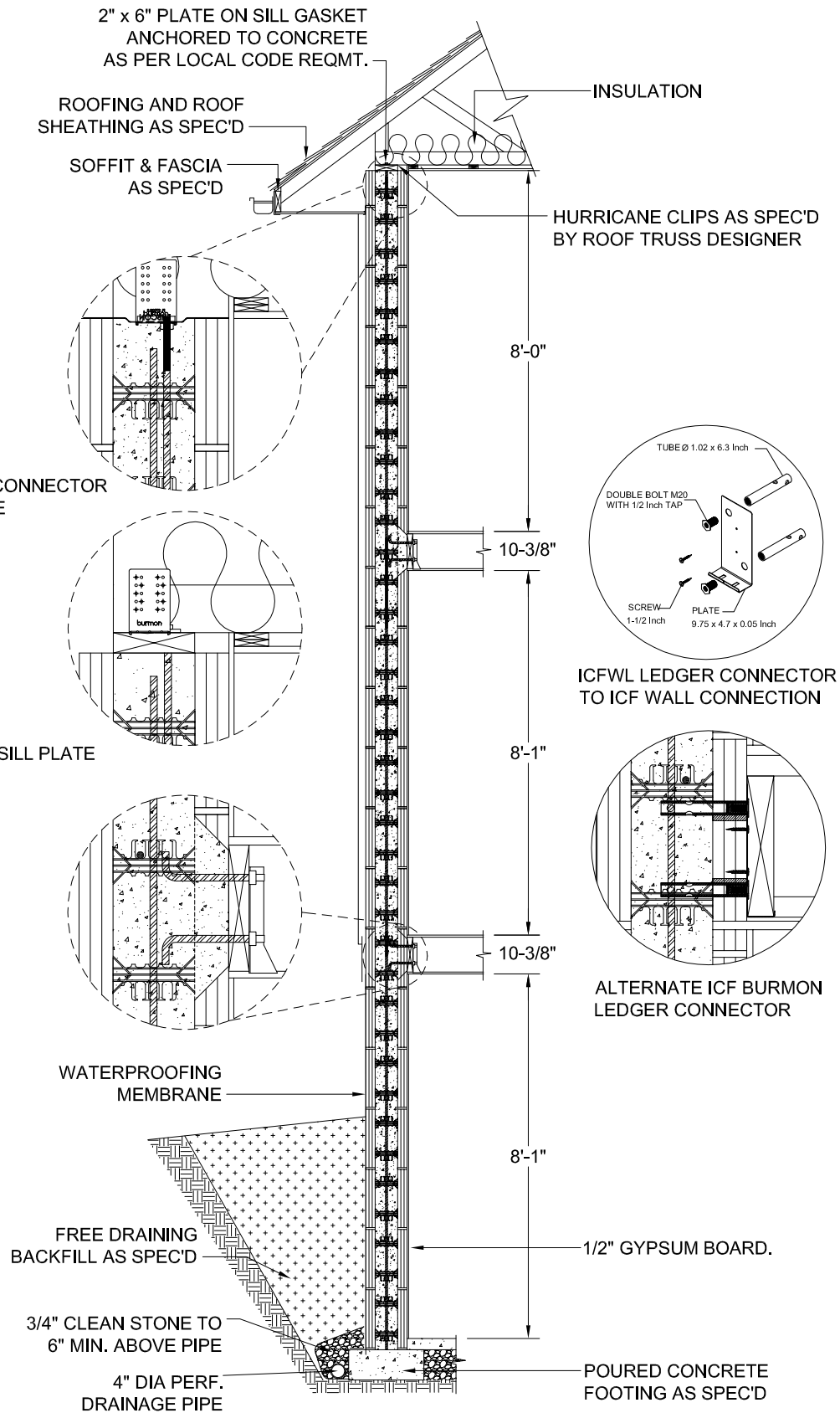
1 WALL SECTION 2 STORY ABOVE GRADE 6 INCH
