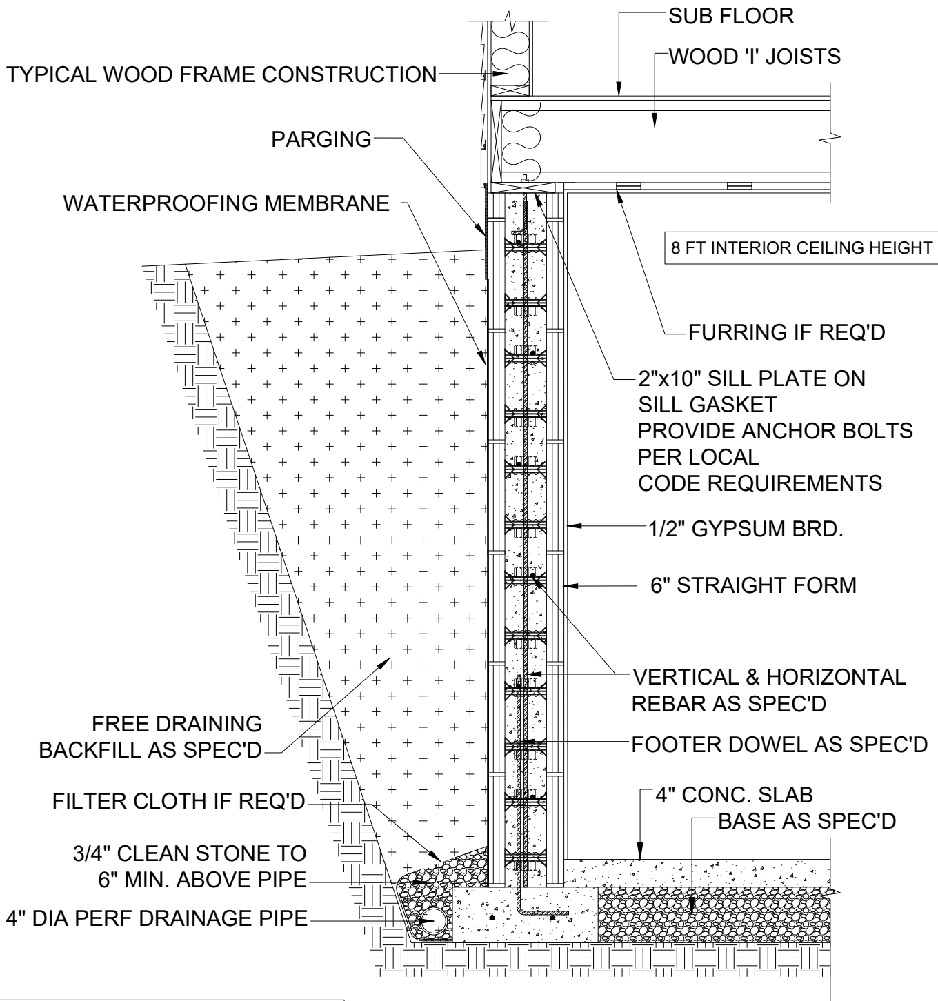
1 TYPICAL FOUNDATION 8' HIGH 6 INCH
