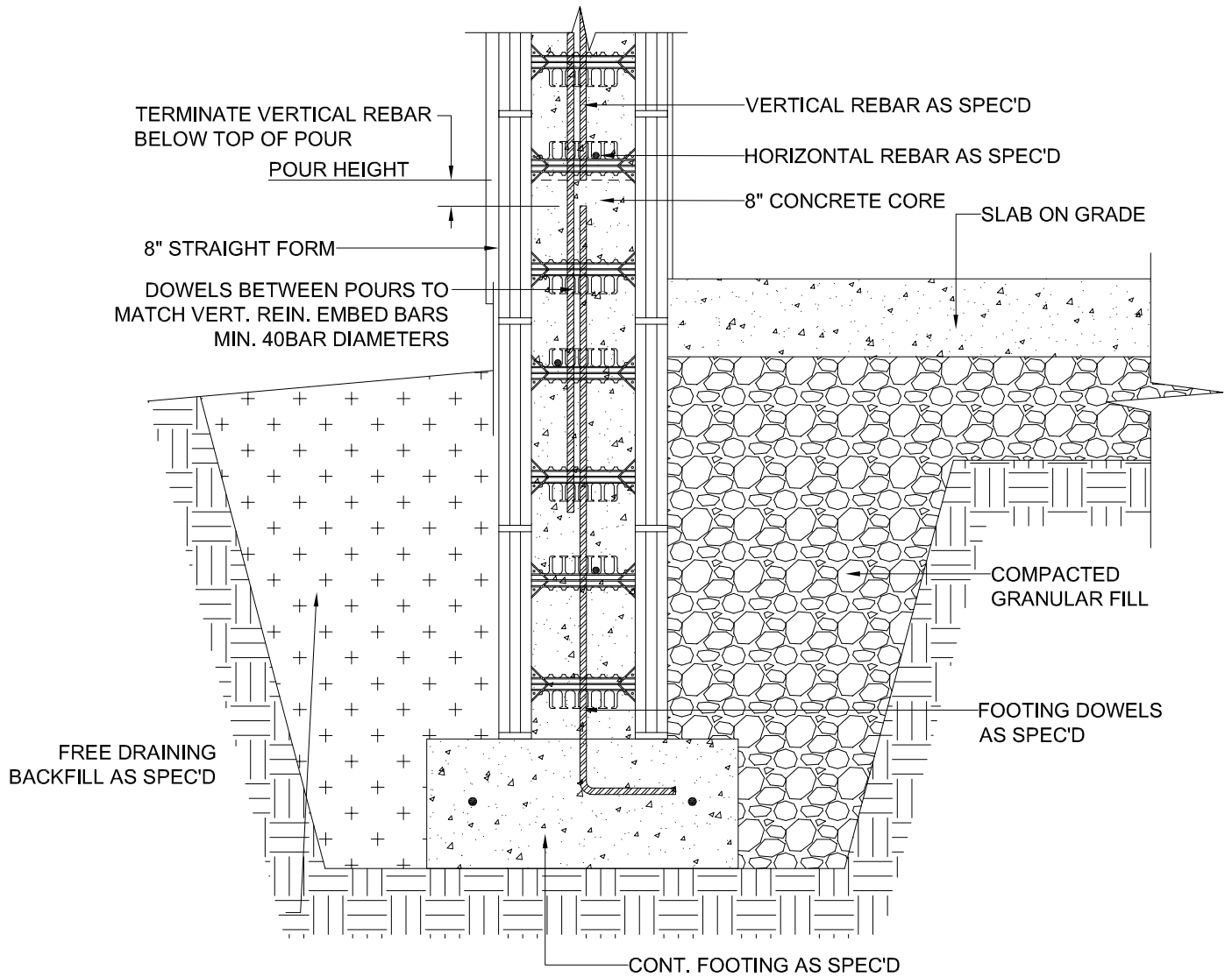
1 STEM WALL INTERIOR SLAB ON GRADE 8 INCH
