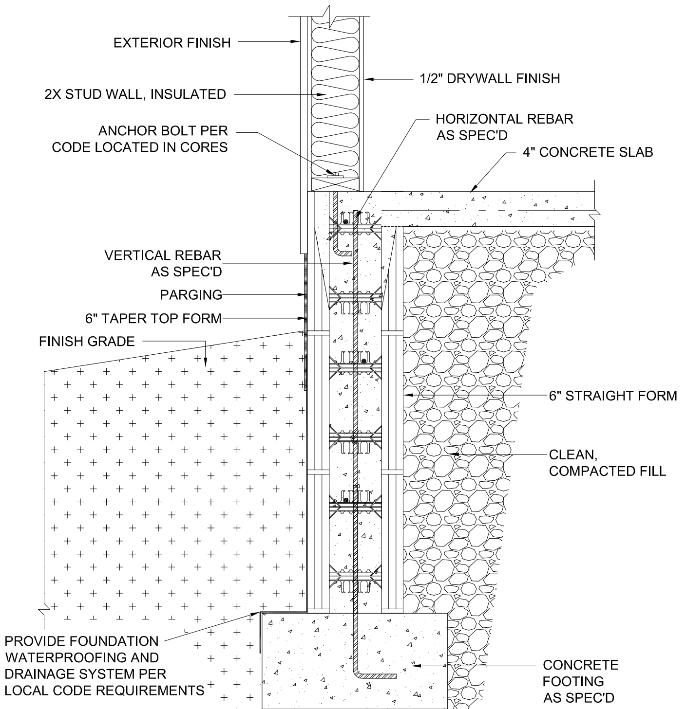
1 SLAB ON GRADE STEM WALL 6 INCH
