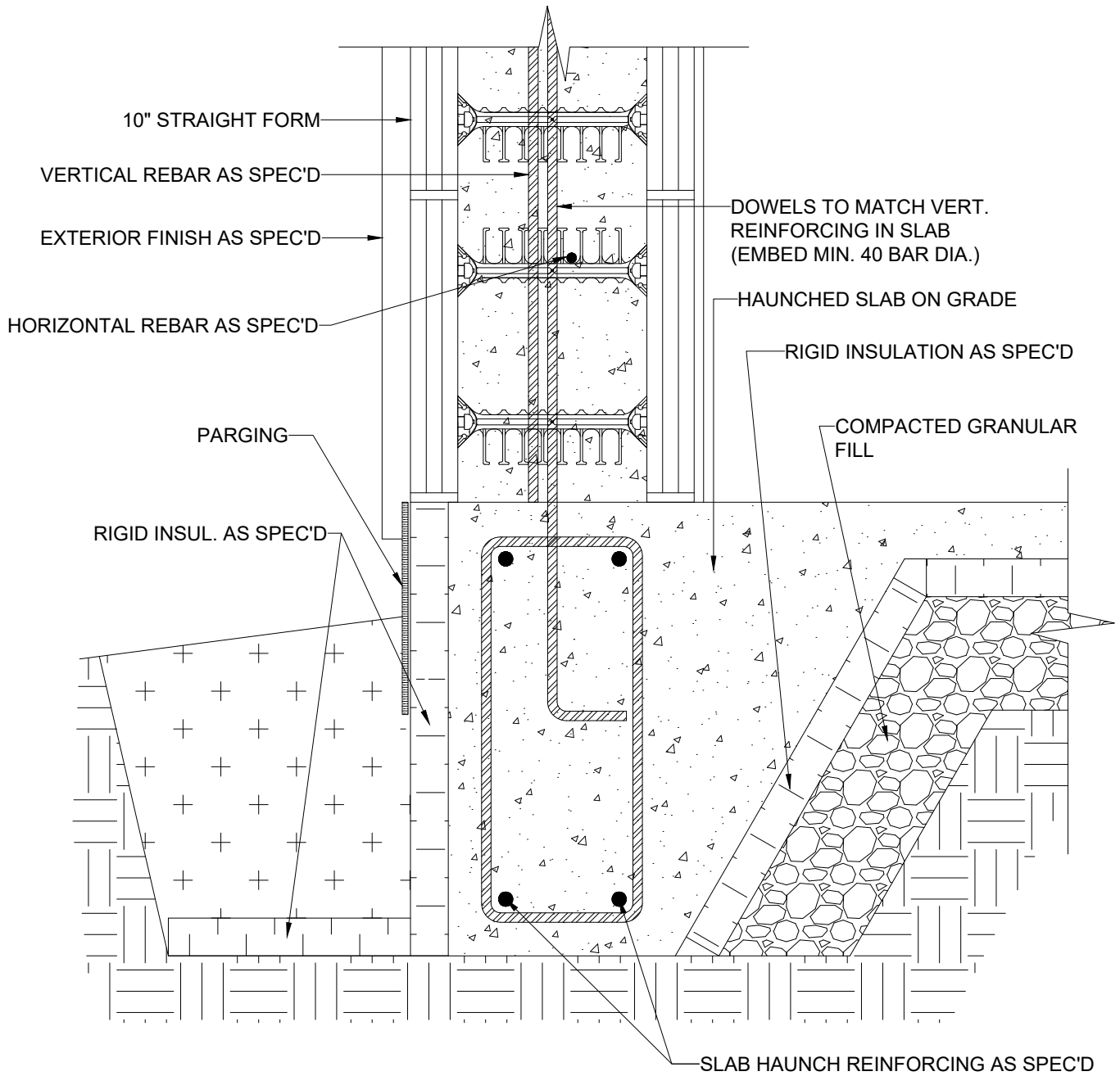
1 HAUNCHED SLAB ON GRADE 10 INCH
