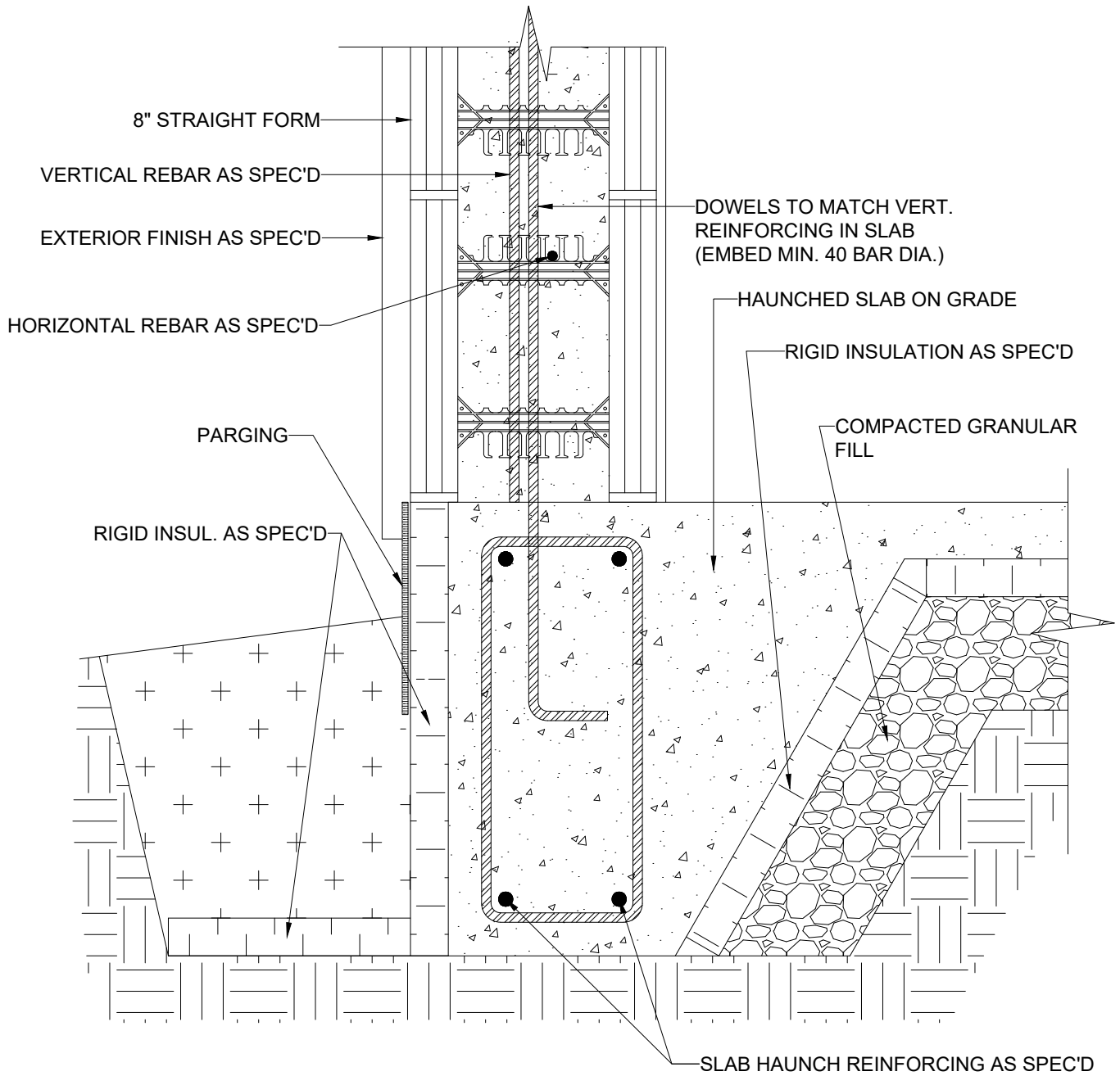
1 HAUNCHED SLAB ON GRADE 8 INCH
