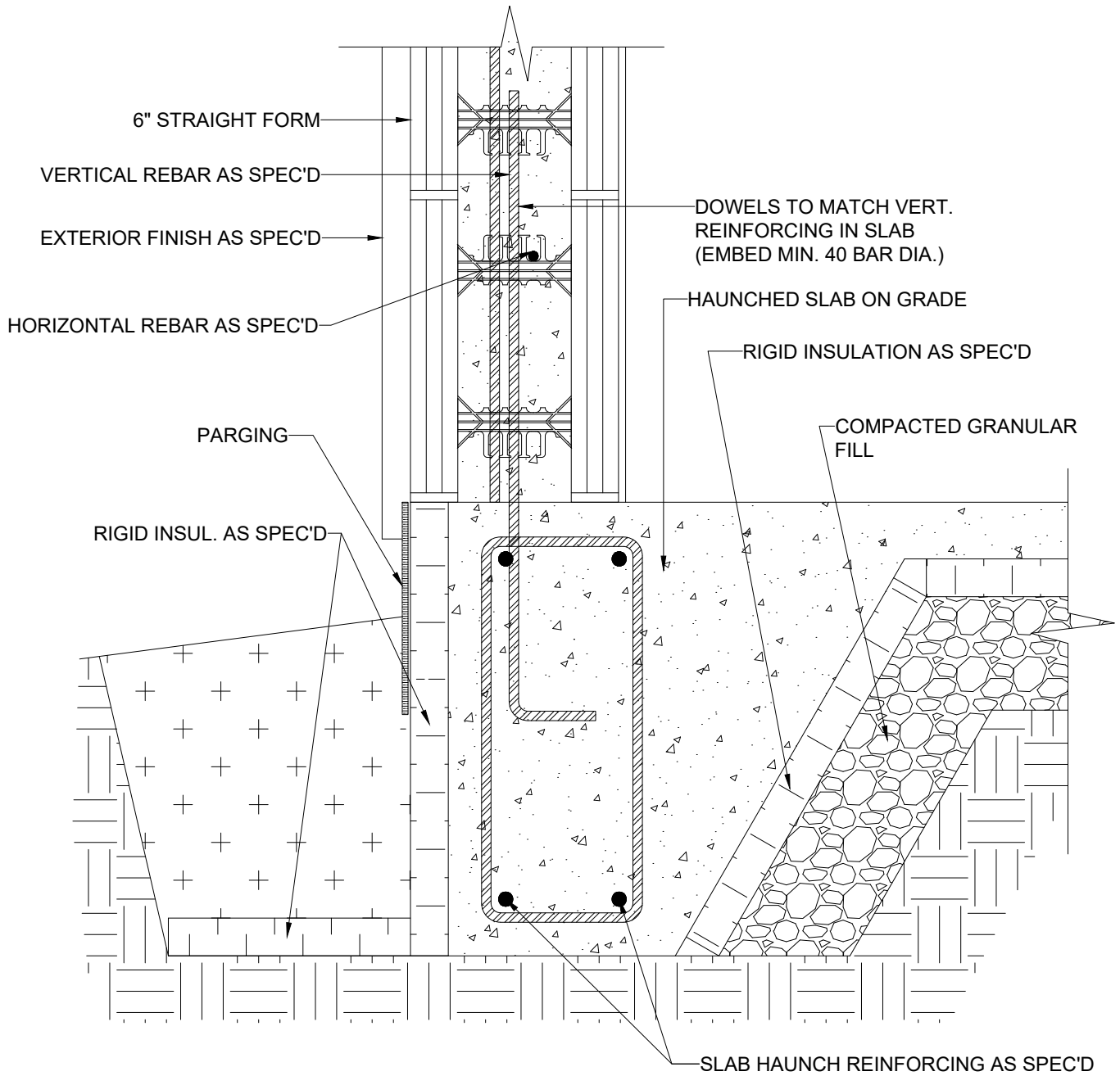
1 HAUNCHED SLAB ON GRADE 6 INCH
