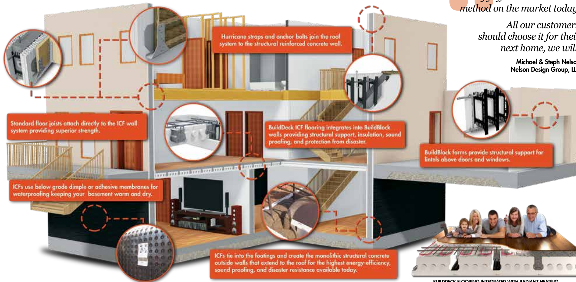
BUILDECK FLOORING INTEGRATED WITH RADIANT HEATING.
