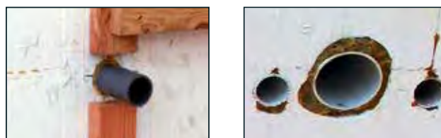
Figure 7.1.5 Add additional strapping if necessary, cut pipes flush after the pour for a seamless finish.
