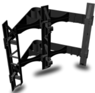
BUILDLOCK CORNER BLOCK WITH BUILDLOCK CORNER WEB HIGHLIGHTED
