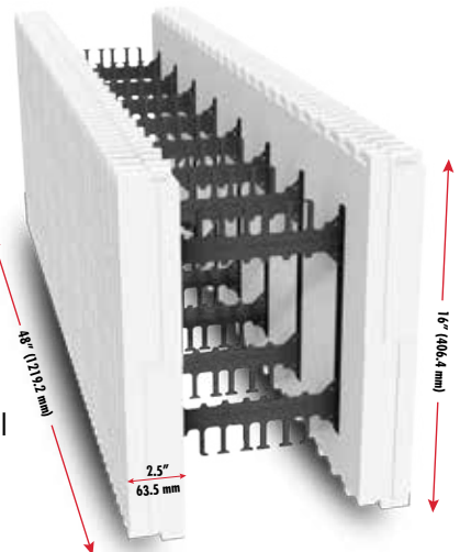
Figure 1.1.1 8-inch Straight Form Shown
