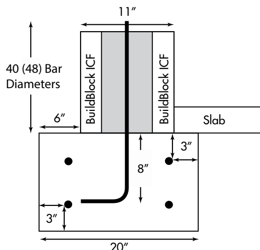
ICF Footing Example using BuildBlock BB-600 6" forms. ACI 318 requires all rebar in concrete touching soil have at least 3-inches of concrete cover.
