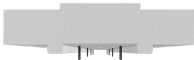
Figure 1.3.9 BuildBuck end view showing factory connection and plastic "T" anchors that embed into the concrete securing the buck to the wall.
