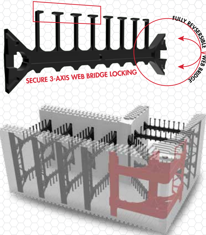
BUILDBLOCK CORNER BLOCK WITH BUILDBLOCK CORNER WEB HIGHLIGHTED
